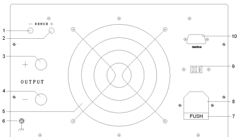
Diagram of rear panel
